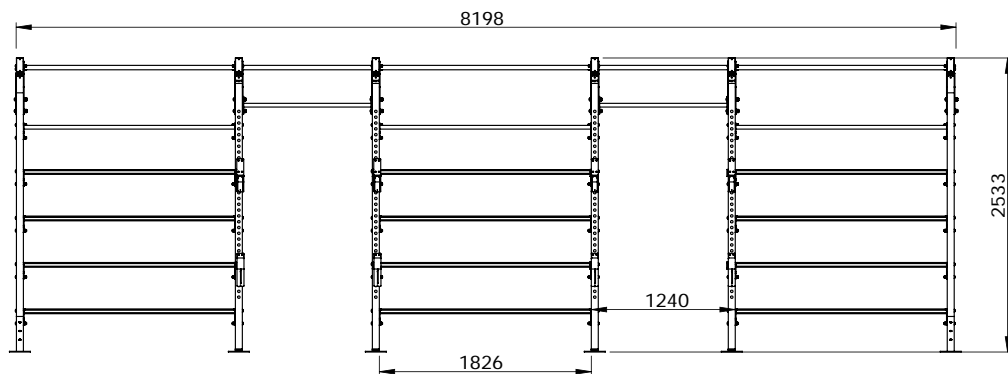
Order Code Item Description ZXP-SSRG-0397-BK XP Floor-Mounted 3x Functional Racks + 2x Squat Bays
