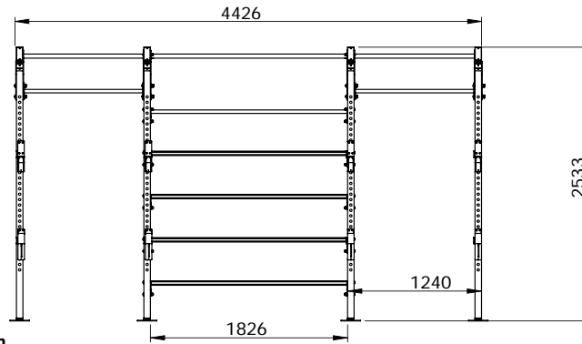
Order Code Item Description ZXP-SSRG-0688-BK XP2 Floor-Mounted 1x Functional Racks + 2x Squat Bays
