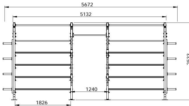
Order Code Item Description ZXP-SSRG-0788-BK XP2 Floor-Mounted 2x Functional Racks + 1x Squat Bays
