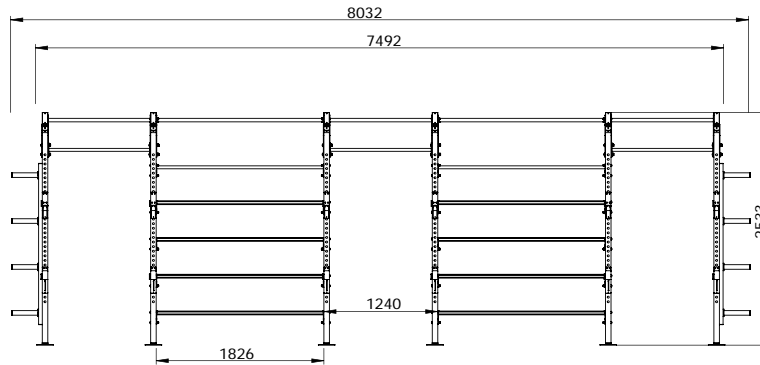
Order Code Item Description ZXP-SSRG-0787-BK XP2 Floor-Mounted 2x Functional Racks + 3x Squat Bays
